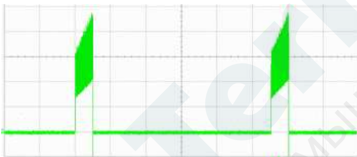
Locked rotor current @ 24 V ( I = 500\text{mA/div} ; t = 1\text{s/div} )
